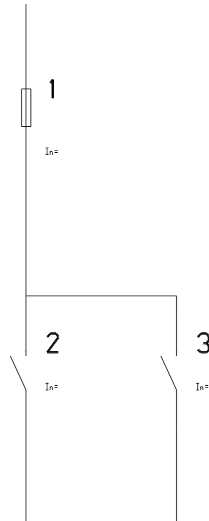
FUKA\KA - 2 MODULY
